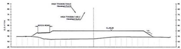
(C) SECTION SCALE 1:500
