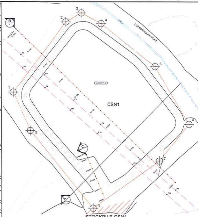
STOCKPILE CSN1 SCALE 1:500
